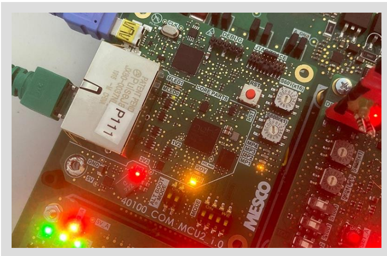
MESCO Evaluation Board PROFINET / PROFIsafe
